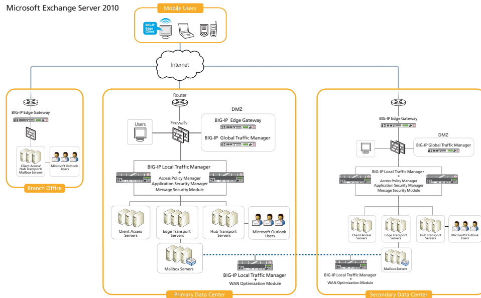
Deployment architecture for complete F5 solution for Exchange Server 2010
